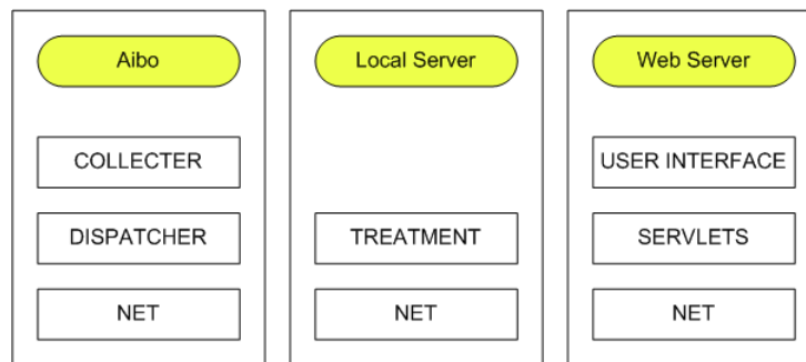
Figure 7.2: Protocol layers
