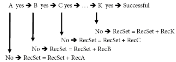
Figure 4 - KBS recommendation mechanism
