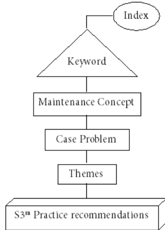
Figure 3 - High-level view of S3^m
