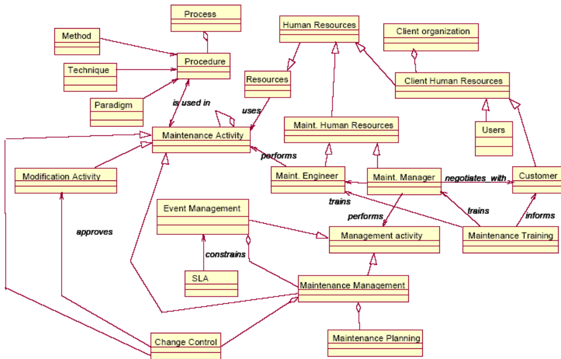
Figure 2 - Part of the software maintenance ontology of (Kitchenham and et al., 1999)
