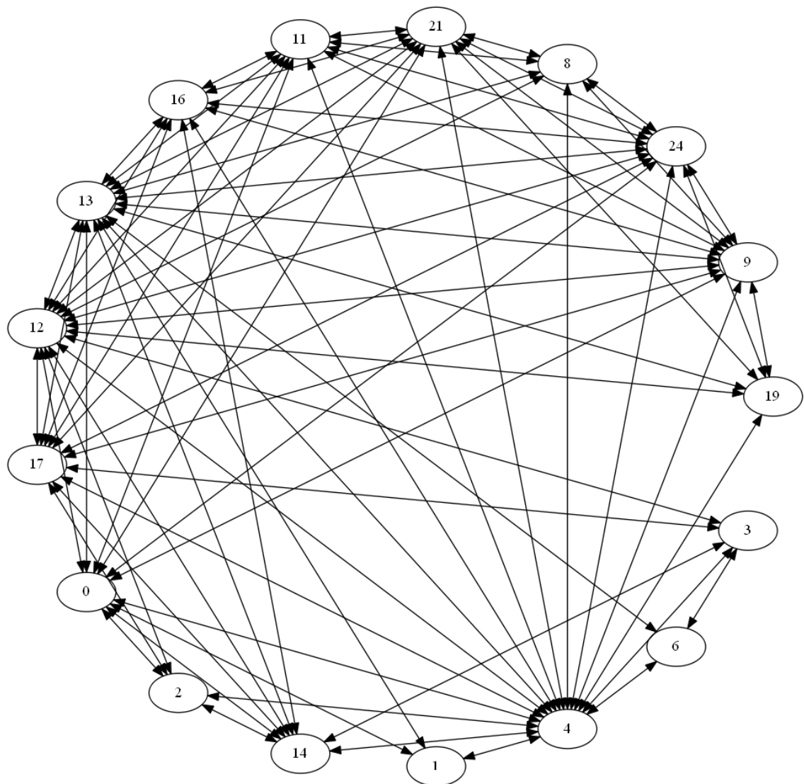
(a) Broadleaf
