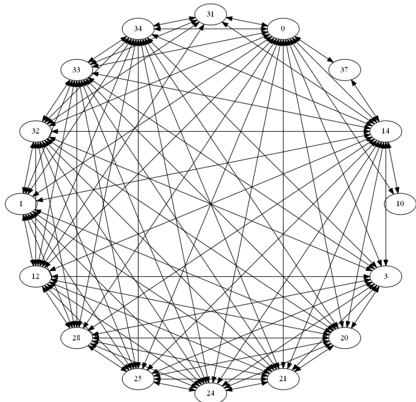
(b) OpenMRS
