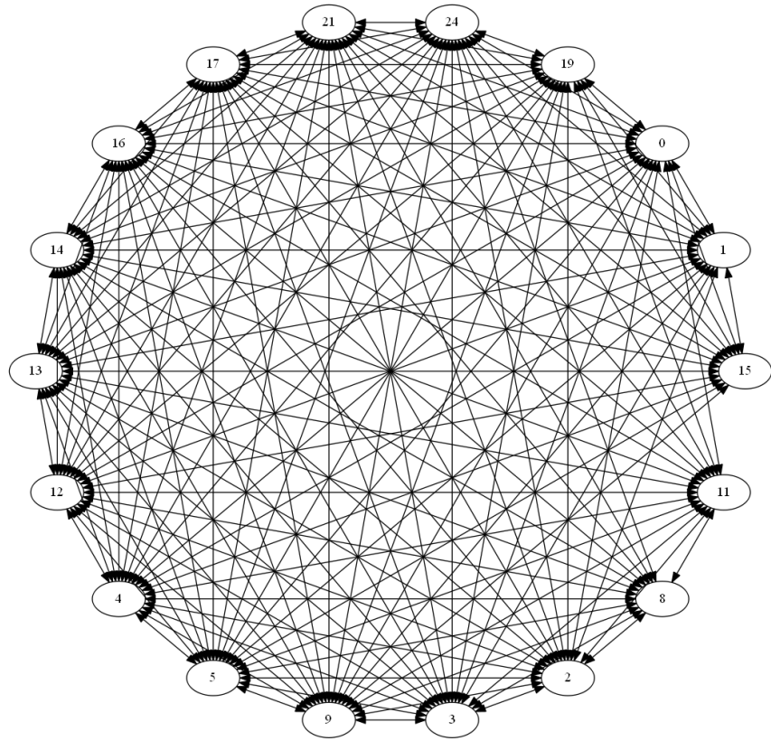
(a) Broadleaf
