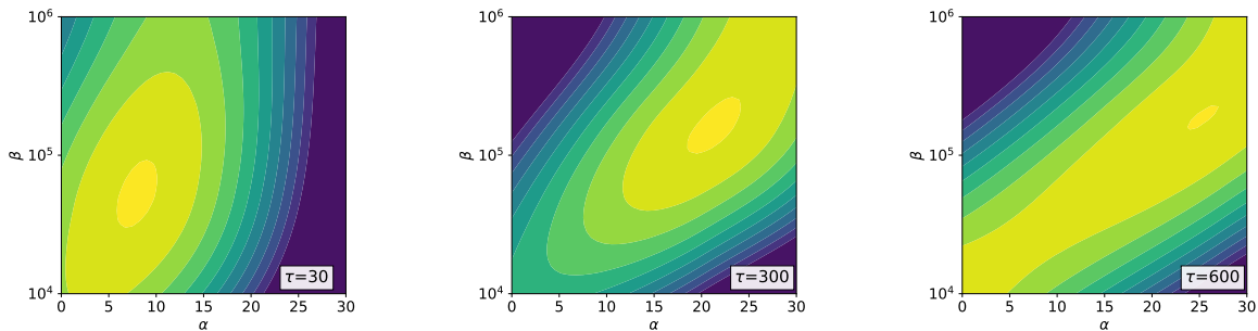
FIG. 3. Contour plots of the log-likelihood function obtained with the GLM timescales \tau = 30, 300 , and 600 seconds. The original data was derived from the nonlinear Hawkes process of the system receiving external fluctuations and self-excitation of the timescale \tau_0 = 300 seconds as in Figure 2(d).
