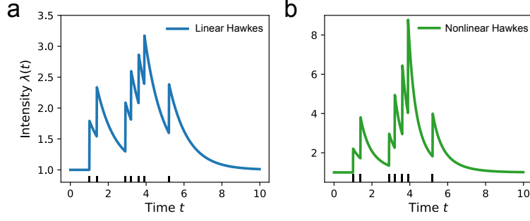
FIG. 1. Comparison of intensity self-reinforcement between (a) the linear Hawkes process and (b) the non-linear Hawkes process. Both processes have background rate equals 1 and exponential memory kernel. We consider the hypothetical situation where events get realised at the same times in each case and compare the resulting intensities. Linear reinforcement generates a constant number of secondary events, while multiplicative effect is stronger if subsequent events arrived closer in time, e.g. around t = 4 .
