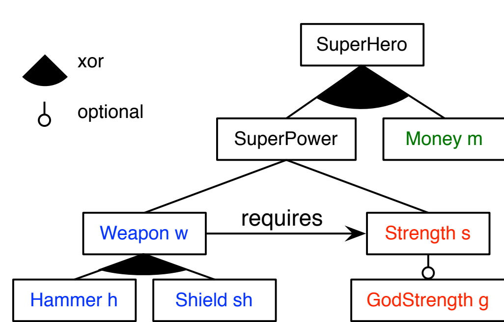
Feature Diagram
