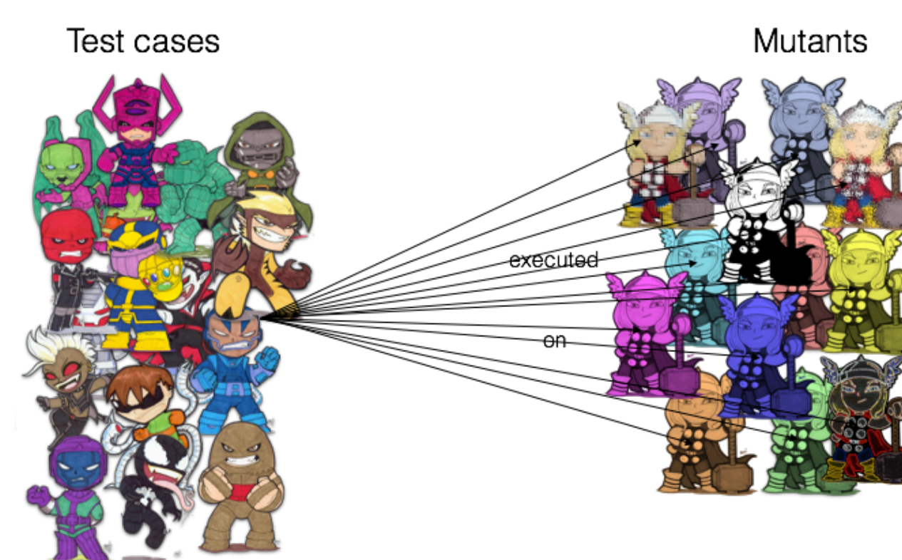
Mutation Testing
