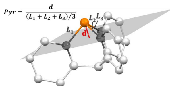
Figure 16 - Measure of the Pyr parameter in the case of phosphatriptycene.
