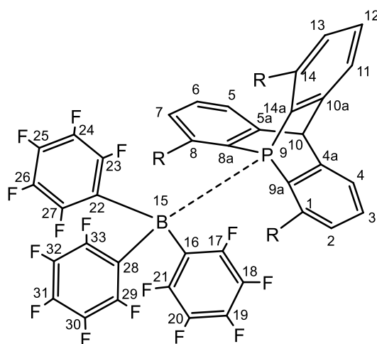
Figure 25 – Shared atomic numbering of all studied compounds.
