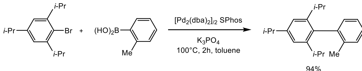
Scheme 3 - Example of a palladium-catalyzed Suzuki-Miyaura cross-coupling reaction with the SPhos ligand.
