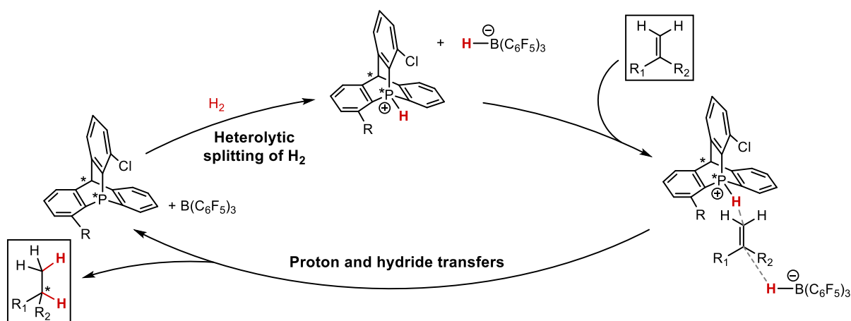
Scheme 44 - Plausible catalytic cycle of enantioselective hydrogenation of alkenes.
