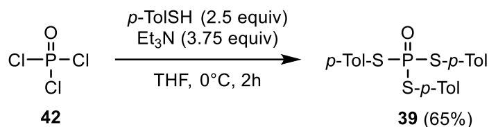
Scheme 29 - Synthesis of phosphine oxide precursor 39.
