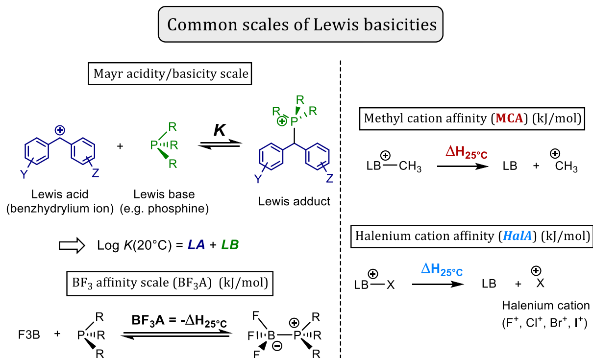
Figure 2 – Common Lewis basicity scales. [15]
