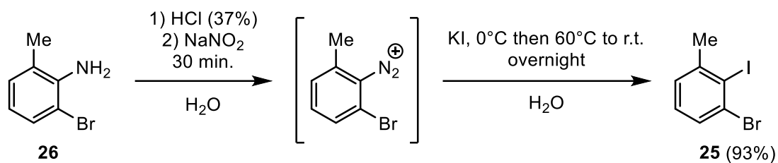
Scheme 22 - Sandmeyer reaction to form 1-bromo-2-iodo-3-methylbenzene ( 25 ) from 2-bromo-6-methylaniline ( 26 ).
