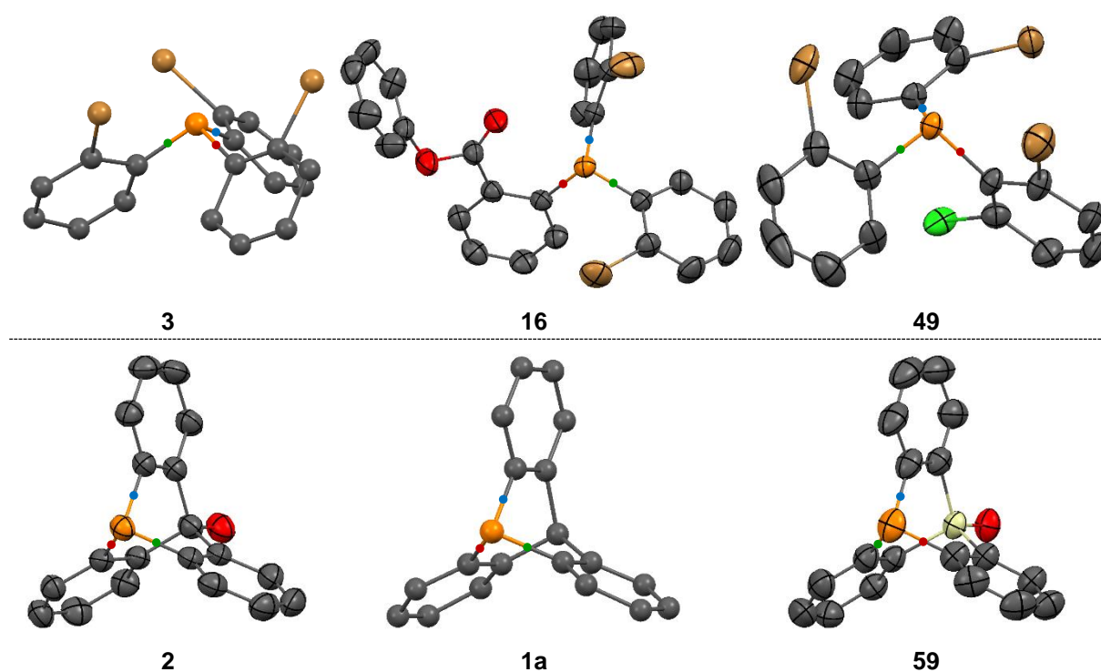
Figure 17 - Molecular structures of compounds 3 , 16 , 49 (classical phosphines), 2 , 1a and 59 (phosphatriptycene derivatives). Thermal ellipsoids are set at 50% probability. Hydrogen atoms are omitted for clarity. The coloured dots refer to the bond lengths indicated in Table 4. Compound 59 was synthesised by Lei Hu in the context of his Ph.D and is shown for comparison purpose.
