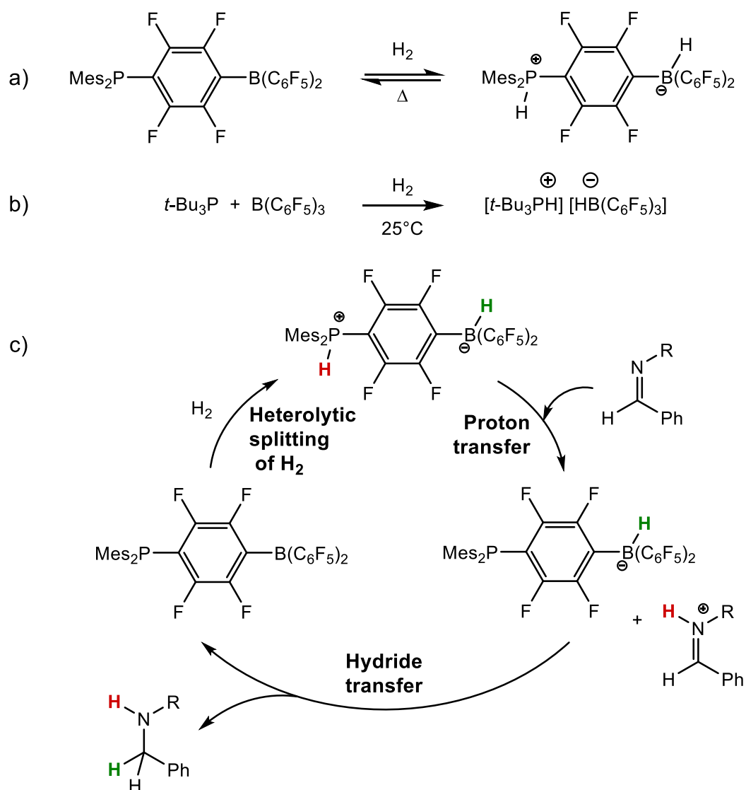
Figure 7 - a) First reversible heterolytic cleavage of \text{H}_2 by a FLP; b) Hydrogen splitting by a borane/phosphine system; c) Catalytic cycle of the reduction of an imine by a FLP.
