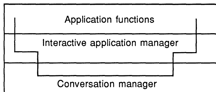
Figure 5.6 : Internal control in interface-application translation.
