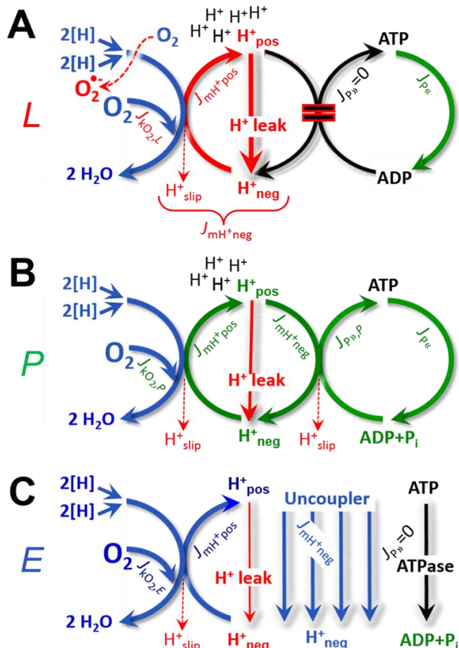
(C) ET-state and rate, E : Oxidation only, since phosphorylation is zero, J_{P\gg} = 0 , at optimum exogenous uncoupler concentration when noncoupled respiration, J_{kO_2,E} , is maximum. The F-ATPase may hydrolyze extramitochondrial ATP.
