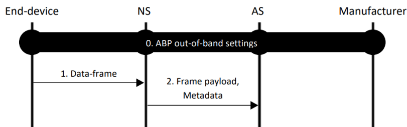
FIGURE 1.5 – Activation d'un device ABP
