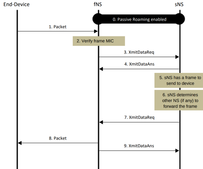
FIGURE 2.6 – Transmission d'un packet en Roaming passif stateful
