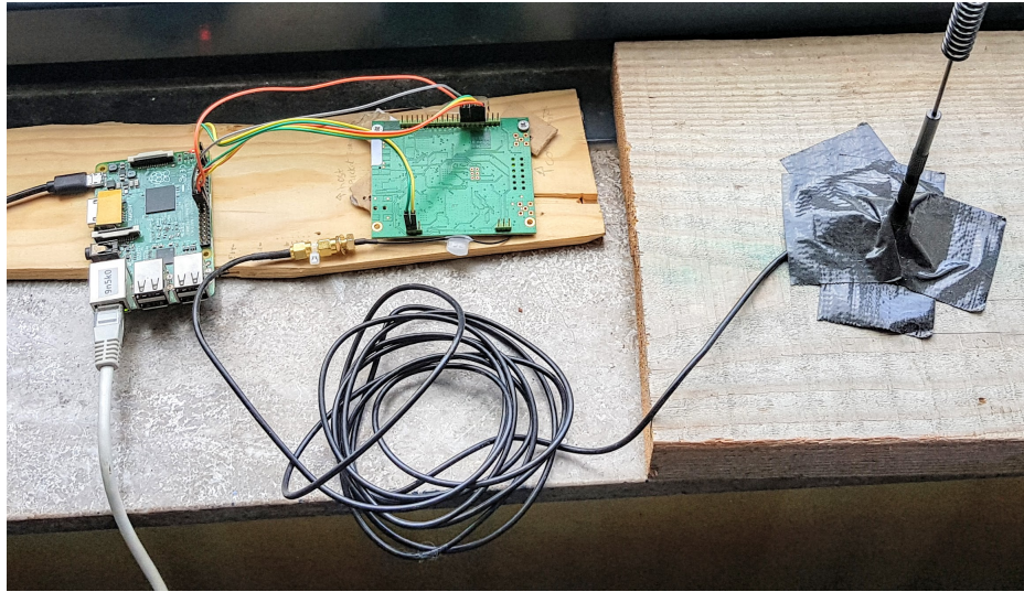
FIGURE 4.3 – Gateway LoRa
