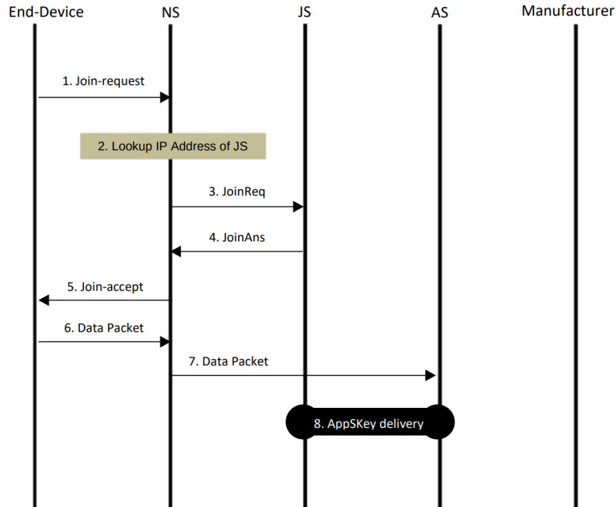
FIGURE 1.6 – OTA Activation
