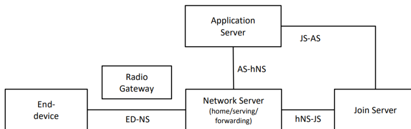
FIGURE 1.4 – LoRaWAN Network Reference Model, End-Device at home[14]
