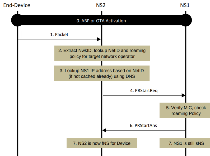
Figure 7 Passive Roaming start
