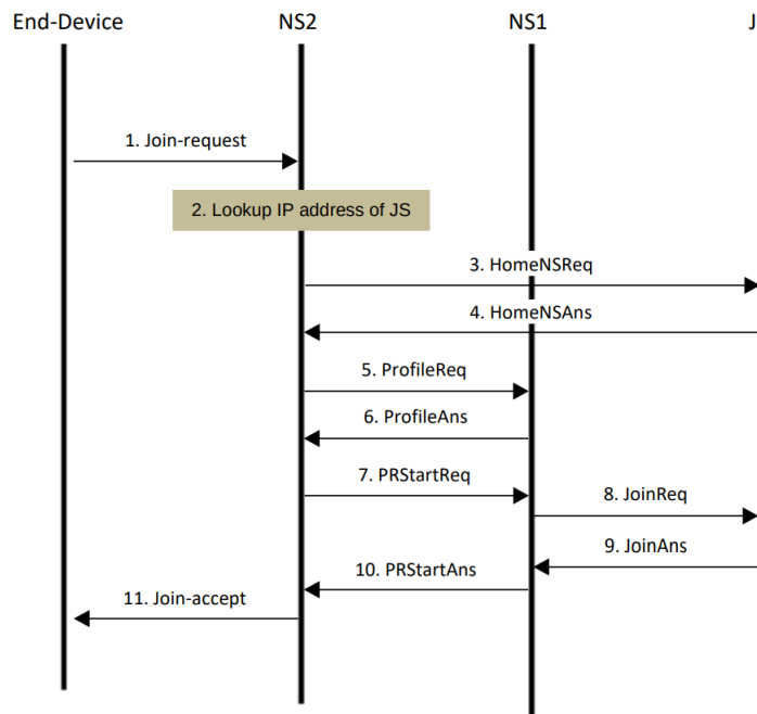
FIGURE 2.5 – OTAA passive Roaming
