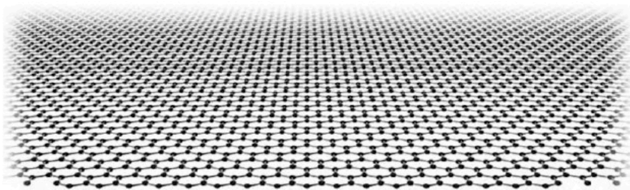
Figure 7. Le graphène
