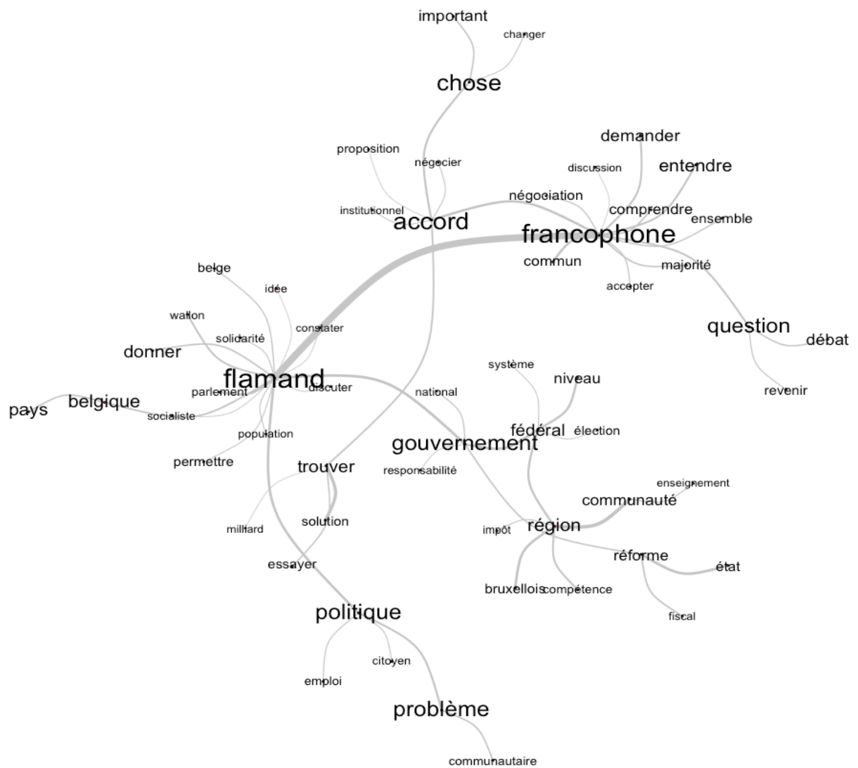
Figure 1: Co-occurrences tree
