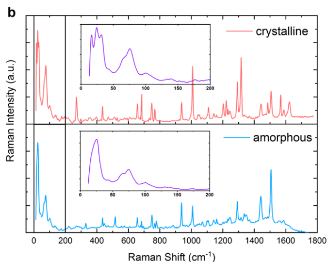
Figure 1: a X-ray diffraction of crystalline and amorphous CMA1. Three distinct peaks appear at 8.2, 8.7 and 10.3 degrees. The inset shows weak crystallisation of annealed PEO (100,000) with two peaks at 19.2 and 23.4 degrees. b Raman spectra of crystalline and amorphous CMA1. Raman shift below 200\text{ cm}^{-1} is magnified. Films were drop cast from CMA1 chlorobenzene solution (20 mg/ml) mixing with 20 wt.% PEO (Mw 100,000 Da) in a nitrogen glovebox, followed by annealing at 120^\circ\text{C} for 1 min to crystallise.
