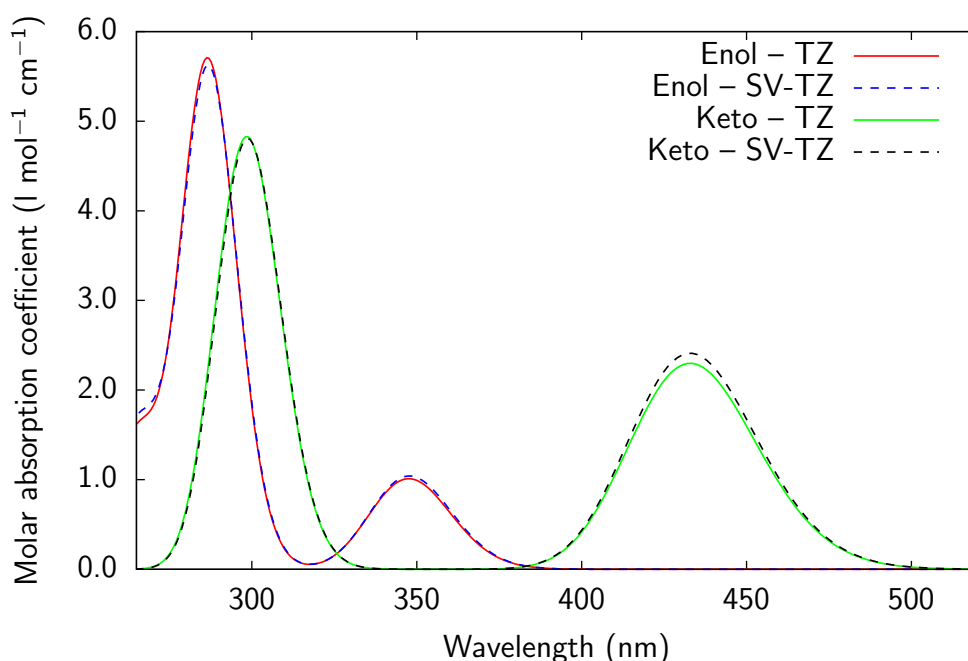
Figure 9. RI-CC2 composite (SV-TZ, dashed lines) and def2-TZVPP (TZ, full lines) spectra for the embedded heteromers of PYV3 · SA and PYV3 · FA1.
