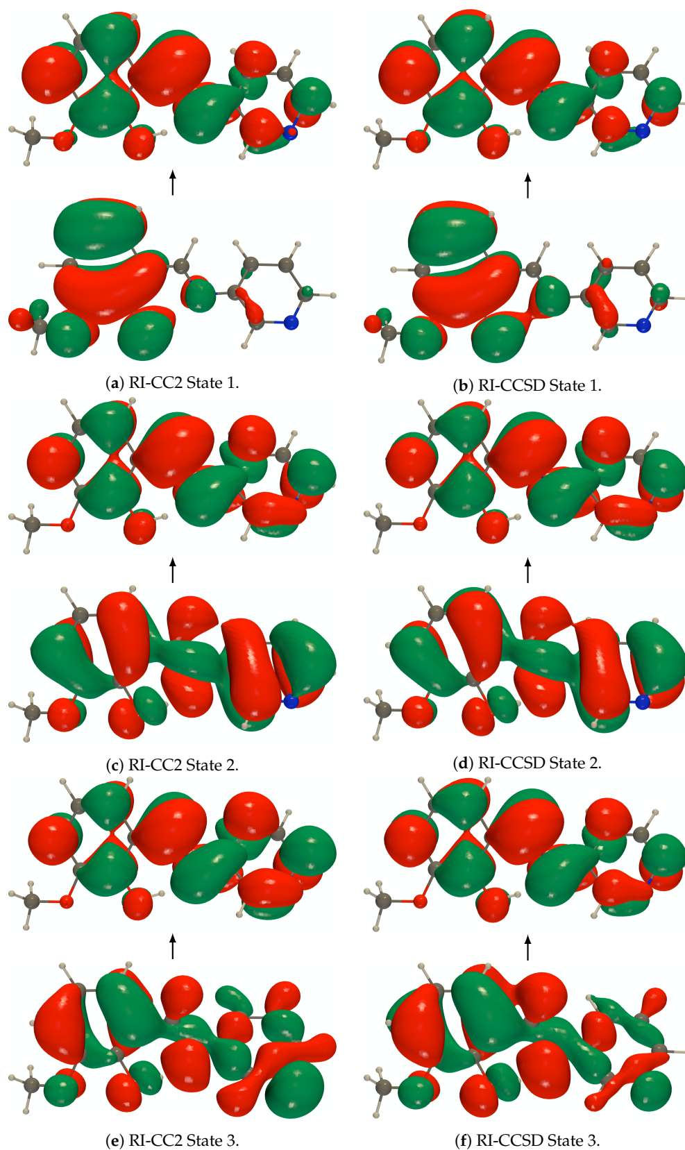
Figure A1. def2-TZVPD NTOs (holes below the arrows and particles above them, the red (green) lobes are the positive (negative) ones) of the isolated PYV3 [PYV3] enol form (isovalue of 0.02 a.u.).
