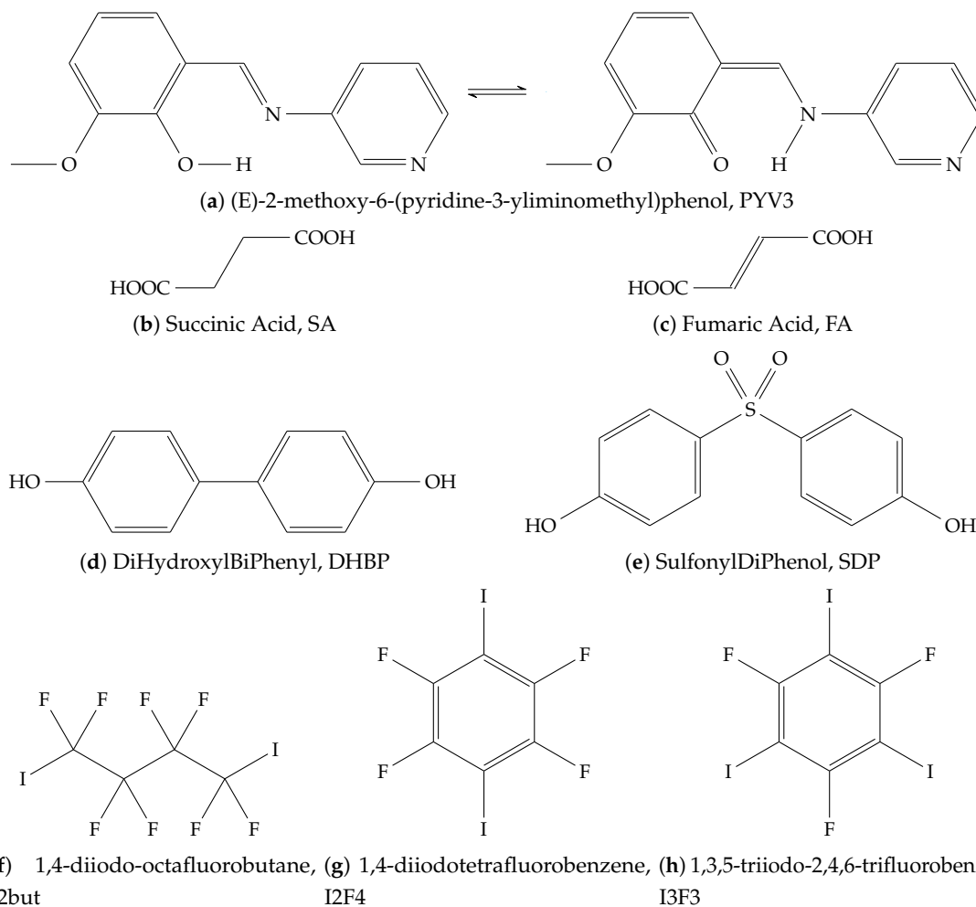
Scheme 1. Structures of PYV3 and its coformers, (a) anil and its enol–keto equilibrium; coformers interacting by H-bond (b–e) or X-bond (f–h).
