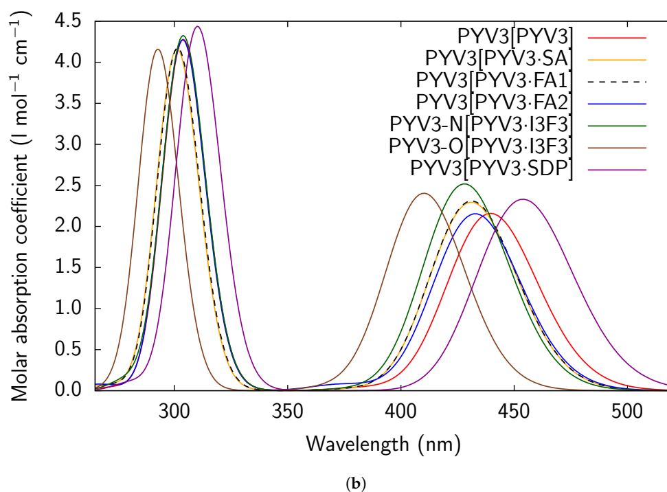
Figure 3. RI-CC2/def2-TZVPD UV/Vis absorption spectra of isolated monomers of all-keto crystals (PYV3 [PYV3 · XXX]). For clarity, the spectra have been splitted in two parts, see (a) and (b).
