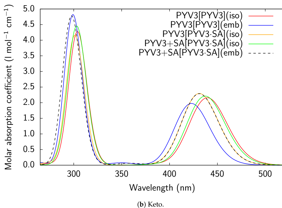
Figure 5. RI-CC2/def2-TZVPD UV/Vis absorption spectra of all models considered for PYV3 and PYV3 · SA.
