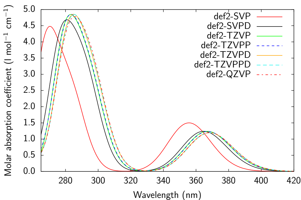
(a) Enol
