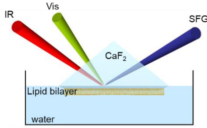
Figure 2. Schematic representation of a SFG measurement at the \text{CaF}_2 /lipid/water interface in a Total Internal Reflection (TIR) geometry of the incident IR and Vis beams and of the generated SFG beam.
