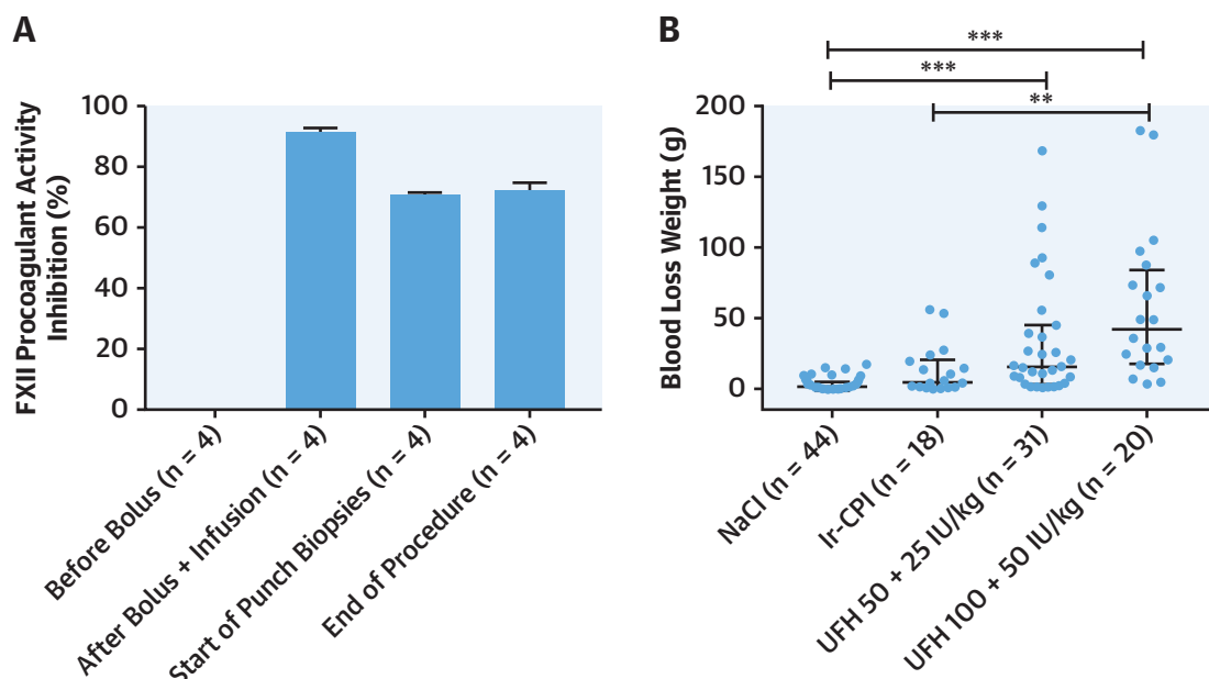
FIGURE 5 Effects of Ir-CPI and UFH on Bleeding
