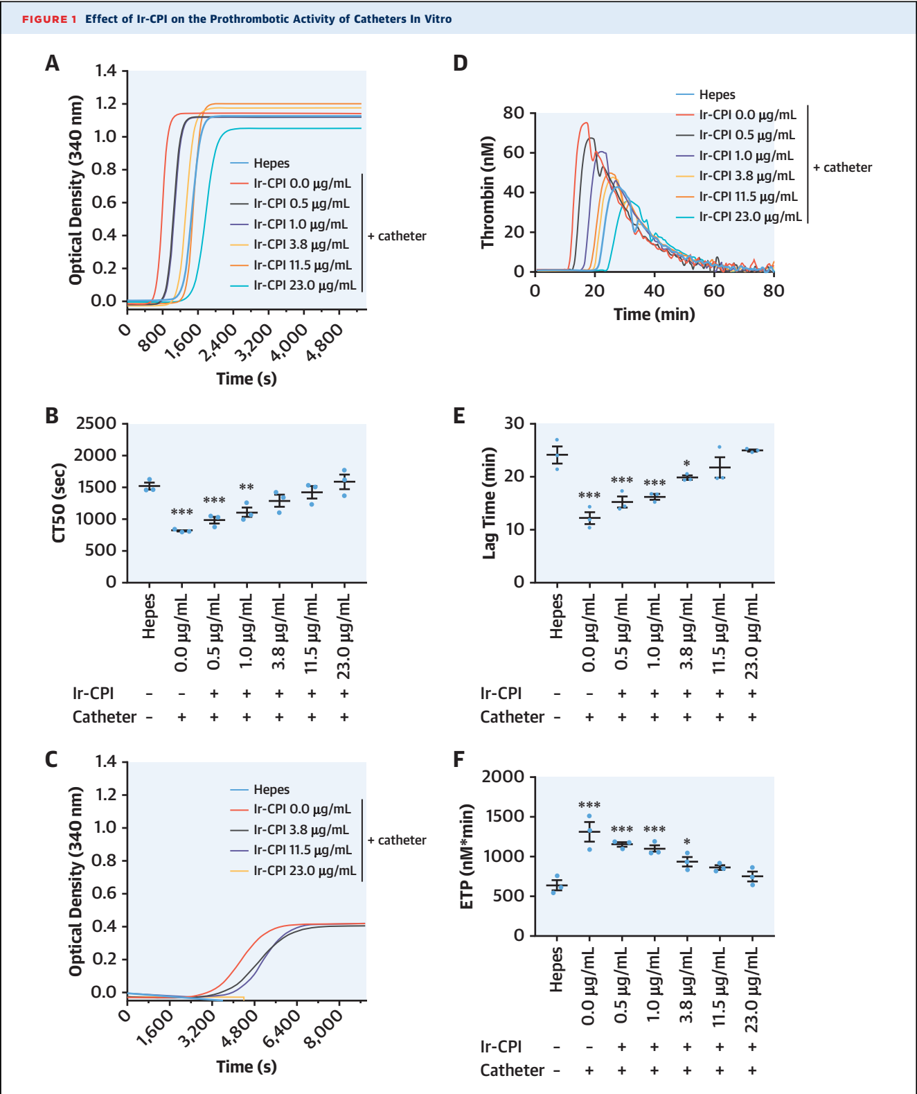
Catheter segments were incubated with platelet-poor plasma (A, B) or factor XII-deficient plasma (C) in wells containing increasing concentrations of Ir-CPI. Clotting was initiated by the addition of \text{CaCl}_2 . (B) Time corresponding to the one-half maximal absorbance was defined as clotting time 50 (CT50). (D) Thrombin generation determination after incubation of catheter segments with platelet-poor plasma. (E, F) Lag time and endogenous thrombin potential (ETP). One-way ANOVA statistical analysis with Dunnett's multiple comparison test was used. * p < 0.05 ; ** p < 0.01 ; *** p < 0.001 . Hepes = 4-(2-hydroxyethyl)-1-piperazineethanesulfonic acid; Ir-CPI = Ixodes ricinus contact phase inhibitor.
