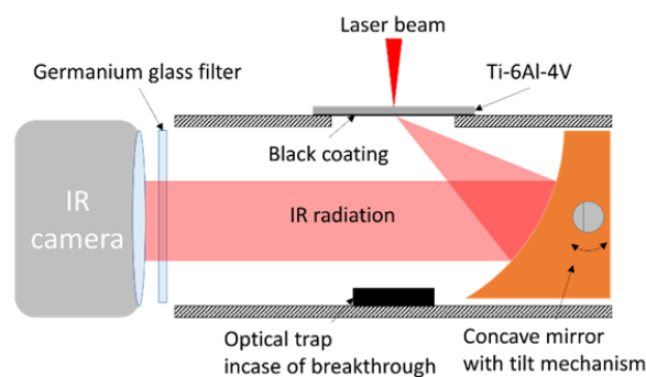
Fig. 2 IR thermography setup
