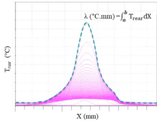
Fig. 6 Demonstration of area under graph ( \lambda )
