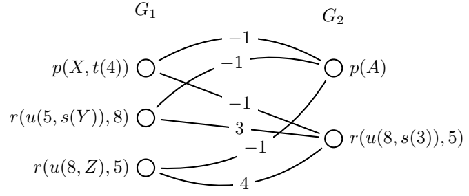
■ Figure 1 The bipartite graph for the assignment problem from Example 20
