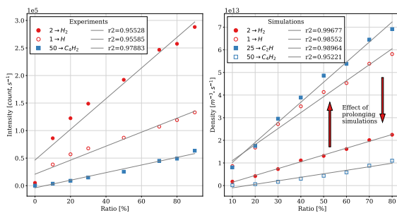
Fig. 3. (Left) Intensity difference ( I_{\text{plasma on}} - I_{\text{plasma off}} ) of main RGA mass spectrometric peaks at 0.02 A, 0.66 Pa, and 10 cm from the cathode with varying acetylene ratio. (Right) Simulation S 1 main radicals' densities after 16 \mu s for different acetylene ratios. The arrows represent the expected relative evolution of concentrations as the reactive H and C 2 H get consumed in reactions producing C 4 H 2 and H 2 .
