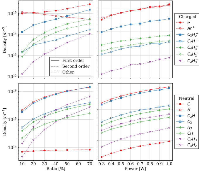
Fig. 10. Mean densities of all charged (Top) and neutral species (Bottom) in the plasma bulk of several simulations after 20 \mu s , with varying acetylene ratio (Left) and power (Right). The different line types are underlying the similar evolutions of several groups of species: the first order (plain), second order (dot-dashed), and other species (dashed).
