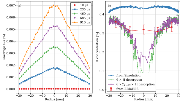
Fig. 9. a-C Coverage (or ratio of DBs) at different timesteps (a) and hydrogen concentration in the simulation with 4% C_2H_2 at 0.8 W (b) with: the average H content in the simulation (blue squares), the hydrogen content in experimentally deposited films from ERDA/RBS measurements (red circles), the hydrogen concentration if the removal of hydrogen from ion impact had a probability multiplied by 6 (green diamonds), and the hydrogen concentration considering the effect of the diminished probability of H desorption in substrate center (purple triangles). (colors online).
