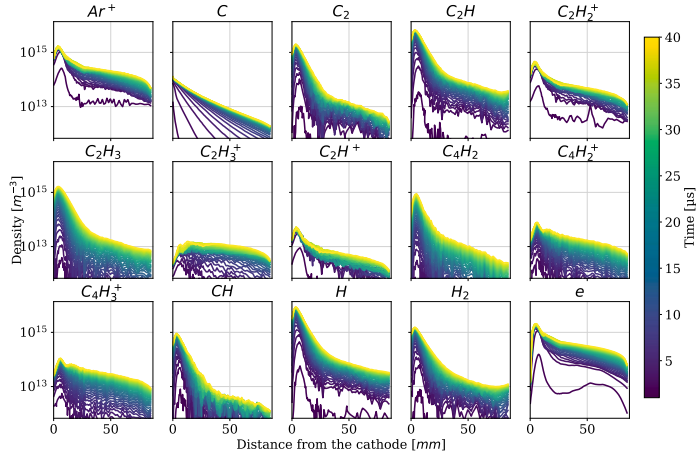
Fig. 7. Mean densities of several species' vs the distance from the cathode surface in millimeters in simulation S_1 (20% acetylene, and 0.8 W). Each curve corresponds to one time-step of 1 \mu s from 0 (blue) to 40 \mu s (yellow). (For interpretation of the references to color in this figure legend, the reader is referred to the web version of this article.)
