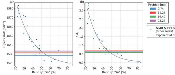
Fig. 3. G peak shift and I_D/I_G ratio vs sp^3 fraction for as-deposited a-CH (data points taken from Ferrari and Robertson [42] and obtained via NMR and EELS measures) fitted with a decreasing exponential function (blue points and gray lines, respectively), as compared to the G peak shifts and I_D/I_G ratios measured on Si27 at different distances from the substrate center (colored ranges with widths corresponding to the fits standard error).
