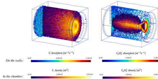
Fig. 8. Carbon and acetylene ion density in the chamber cut with a vertical plane and absorption profiles on the chamber walls in the S_1 simulation after 40 \mu s.
