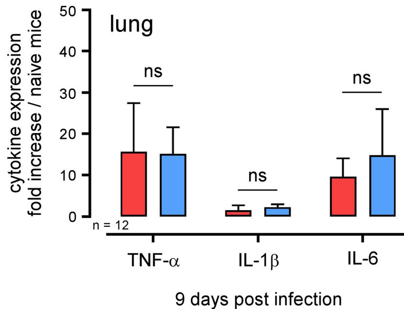
Fig 7. Enhanced susceptibility of B. abortus infected Acod1 -/- mice is not associated with higher pro-inflammatory cytokine expression in the lungs. Wild-type (red) and Acod1 -/- (blue) C57BL/6 mice were intranasally infected with 10 7 CFU of wild-type mCherry expressing B. abortus 2308. At 9 days post infection, mice were sacrificed, lungs were collected, RNA was extracted and qRT-PCR was performed. TNF-α, IL-1β, and IL-6 expression levels were analyzed. Tbp gene was used as negative control, and RNA from naïve mice was used as the standard condition. Data show the fold increase of RNA expression for the indicated cytokine from infected mice compared to control mice. At least 6 mice were pooled for each condition. The data are representative of 3 independent experiments. ns = non-significant.
