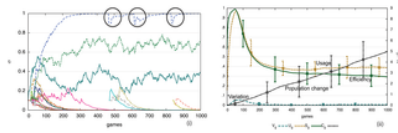
Figure 4. Performance of the formal marker strategy.
