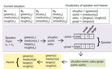
Figure 8. Reuse strategy.
