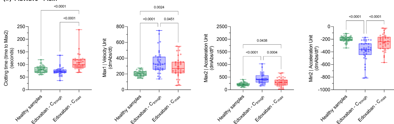
FIGURE 2 Population comparison of activated partial thromboplastin time (A) with the FibIn (B). Only the common parameters of the two tests are presented. C MAX , maximum concentration; C TROUGH , minimum concentration; CWA, clot waveform analysis
