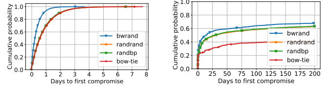
(a) Without client-side guard logic. (b) Enabling client-side guard logic.
