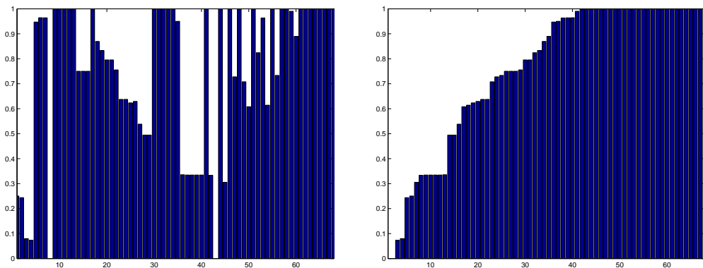
Figure 7.4: The reduction obtained by presolving (for 68 problems with H \neq 0 ) on the number of nonzero entries in H , sorted by decreasing number of such entries in the original problem (left) and by decreasing reduction (right).
