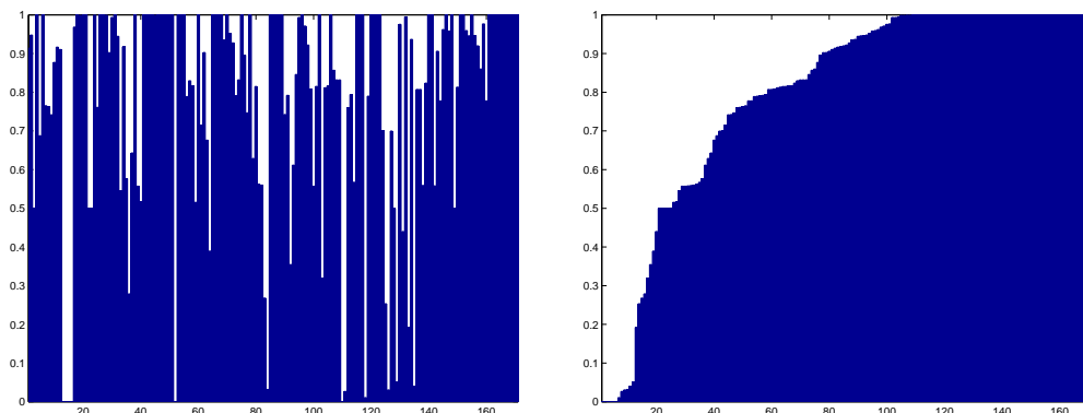
Figure 7.2: The reduction obtained by presolving (for 171 problems with A \neq 0 ) on the number of constraints, sorted by decreasing number of constraints in the original problem (left) and by decreasing reduction (right).
