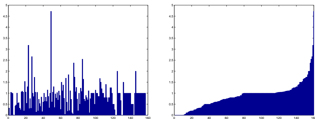
Figure 7.7: The reduction (or increase) of solution time with presolving in loosest mode, sorted by decreasing solution time for the original problem (left) and by decreasing reduction (right).
