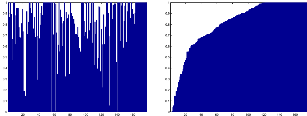
Figure 7.1: The reduction obtained by presolving (for 178 problems) on the number of problem variables, sorted by decreasing original problem size (left) and by decreasing reduction (right)
