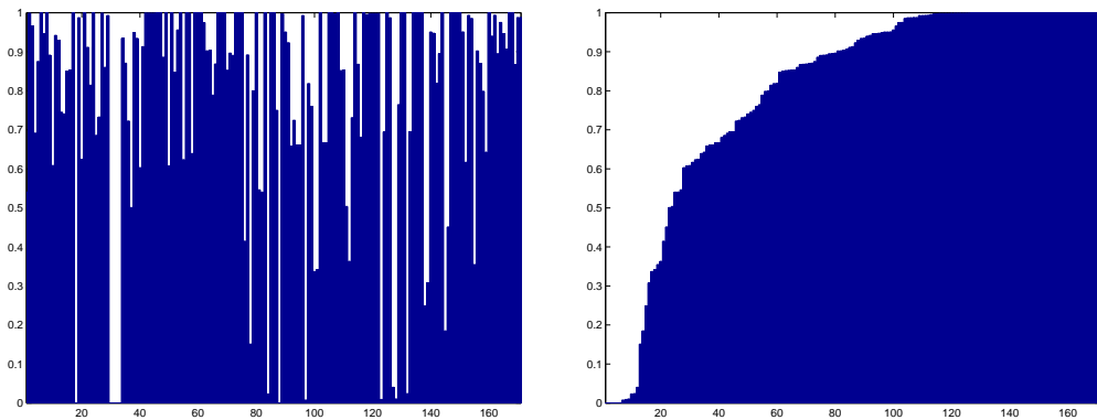
Figure 7.3: The reduction obtained by presolving (for 171 problems with A \neq 0 ) on the number of nonzero entries in A , sorted by decreasing number of such entries in the original problem (left) and by decreasing reduction (right).
