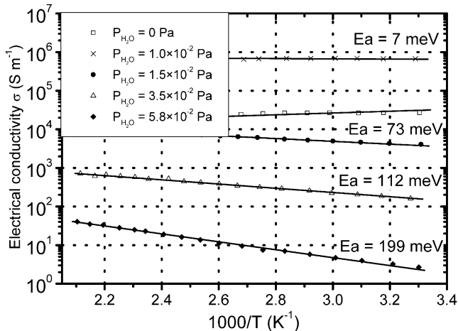
Fig. 9. Electrical conductivity \sigma vs. 1000/T measured on titanium nitride (□) and oxynitride thin films for various water vapour partial pressures. The activation energy E_a (linear behaviour in the Arrhenius plot) is largely influenced by the water vapour partial pressure.
